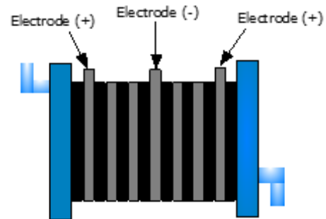
Fig. 7 HHO generator with three electrodes applied
