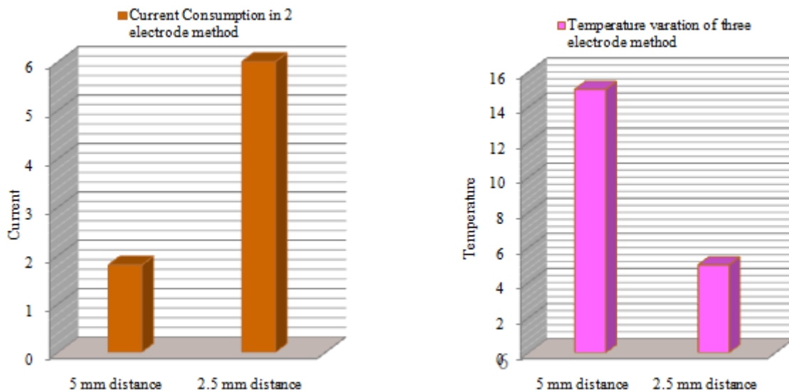
Fig. 11 (a) Maximum flow of current to generate 1 l of HHO, (b) Representation of results in Table - 3
