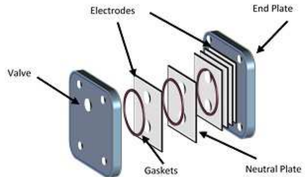
Fig. 4 Dry Cell Concept
