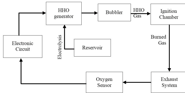
Fig. 13 Block diagram of the Complete System
