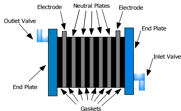
Fig. 5 Cross Sectional view of the proposed HHO generator
