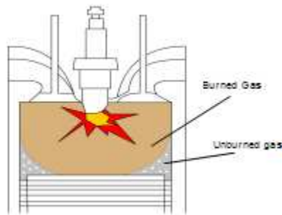
Fig.1 Flame Propagation in the chamber
