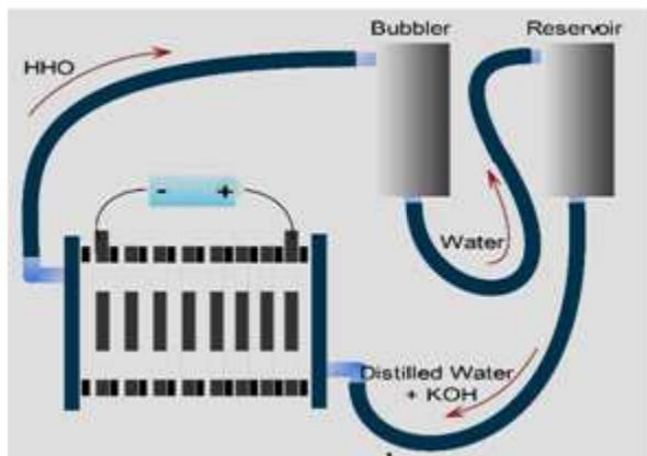
Fig. 6 HHO generator system with bubbler and the reservoir
