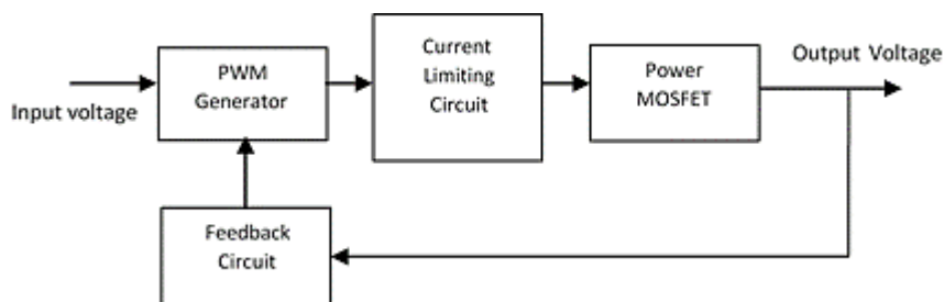
Fig. 12 Block diagram of the Electronic Circuit
