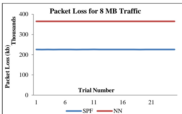
Fig 9 8 Packet losses at the destination when 8 MB of traffic is sent
