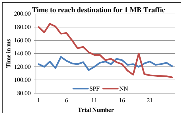
Fig 8 Time to reach the destination when 1 MB of traffic is sent
