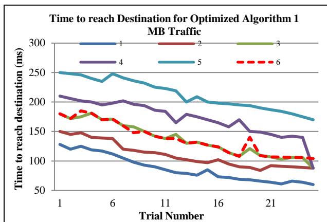
Fig. 12 Time to reach the destination when 1 MB of traffic is sent
