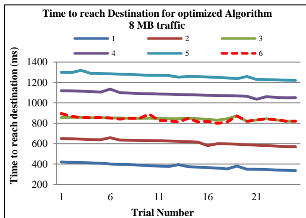
Fig. 14 Time to reach the when 8 MB of traffic is sent.
